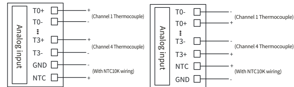
Figure 14 Customized 43C thermocouple wiring
