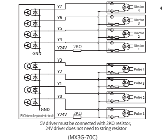
Figure 12 Pulse output wiring
