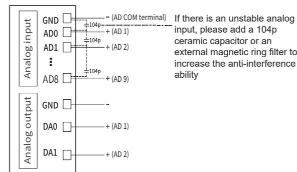
Figure 13 PLC analog wiring
