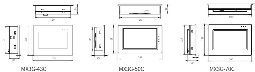
Figure 1 Installation dimension
