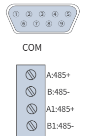
Figure 6 PLC 485 port
