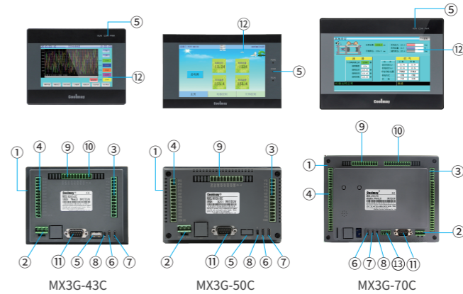
Figure 2 Product structure
